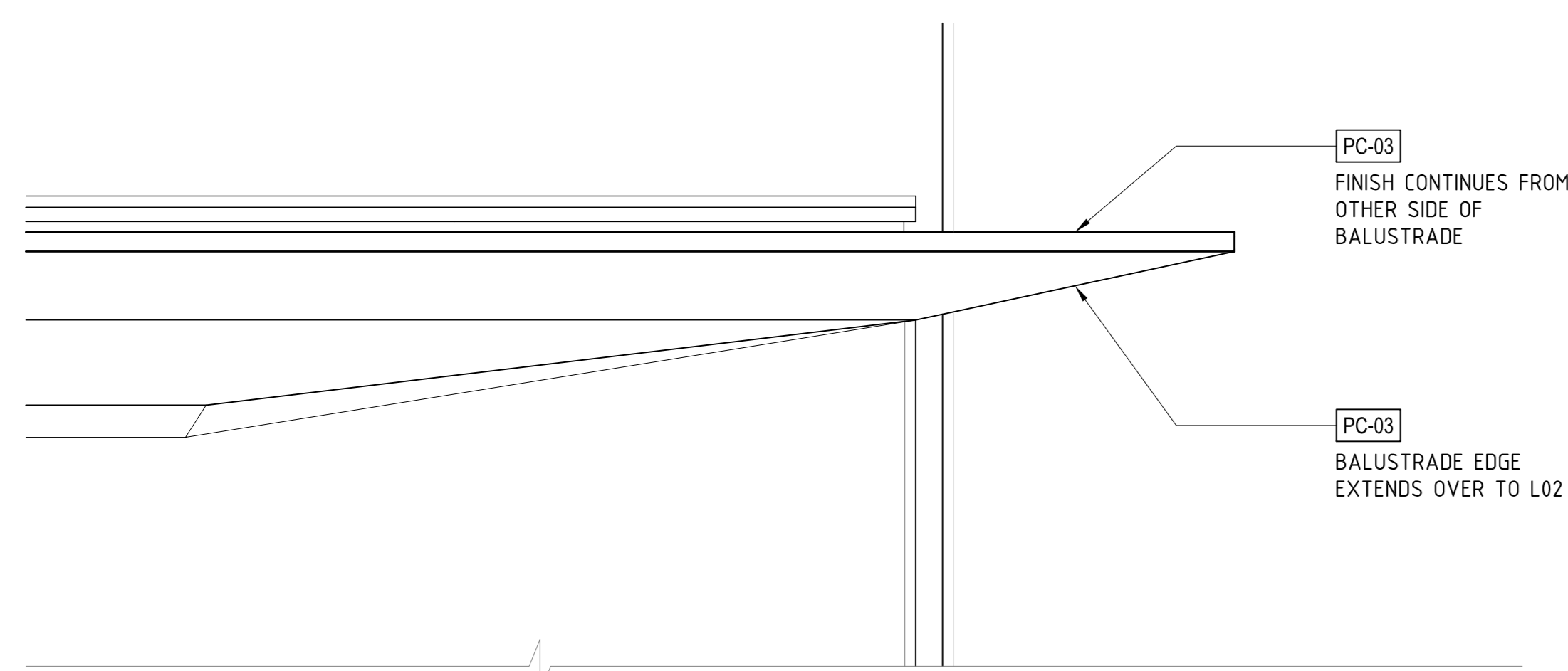
5 JR STUDY SPACE (247) - PLAN DETAIL SCALE 1:5
