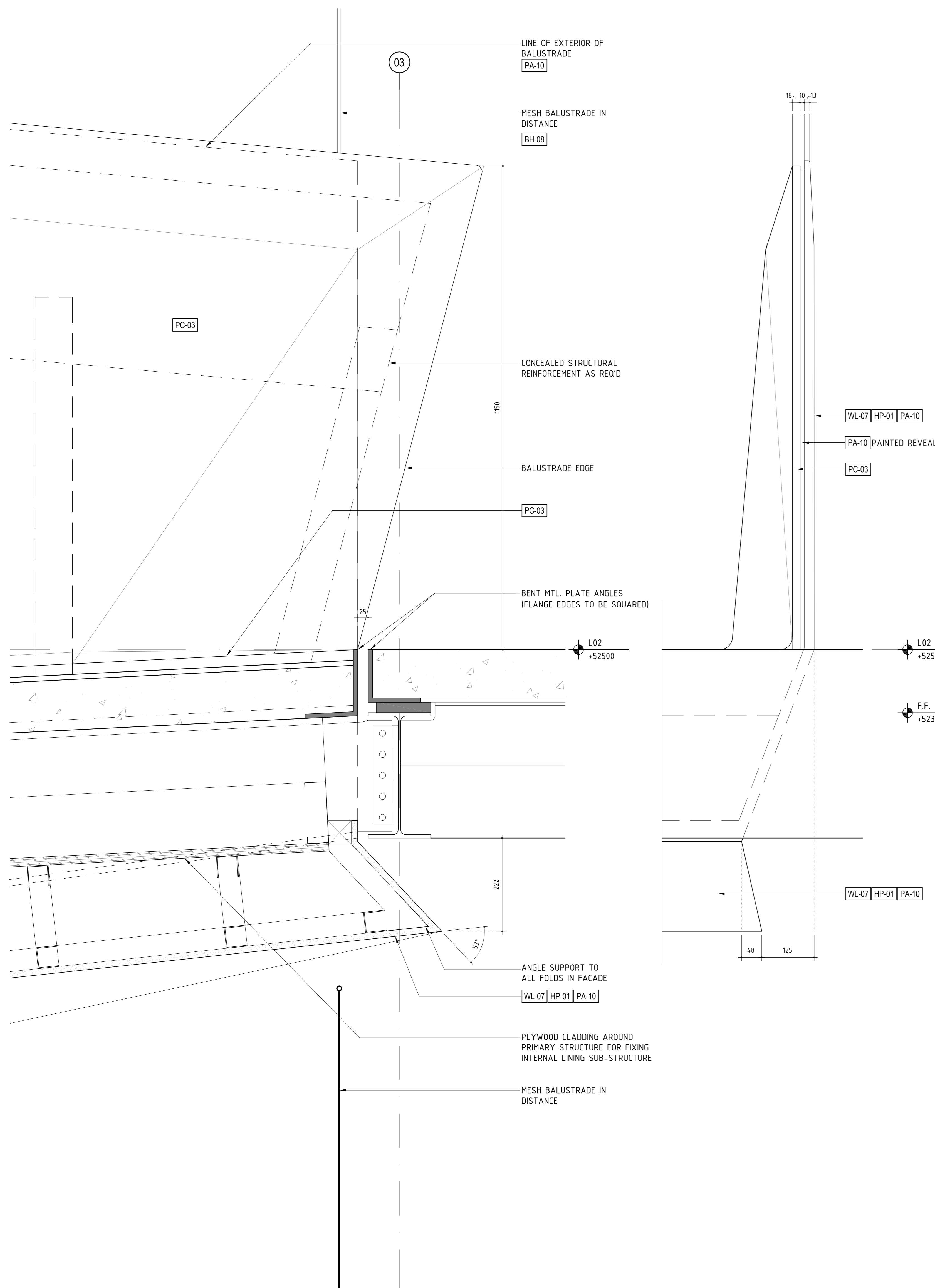
02 JR STUDY SPACE (247) - ELEVATION DETAIL SCALE 1:5
