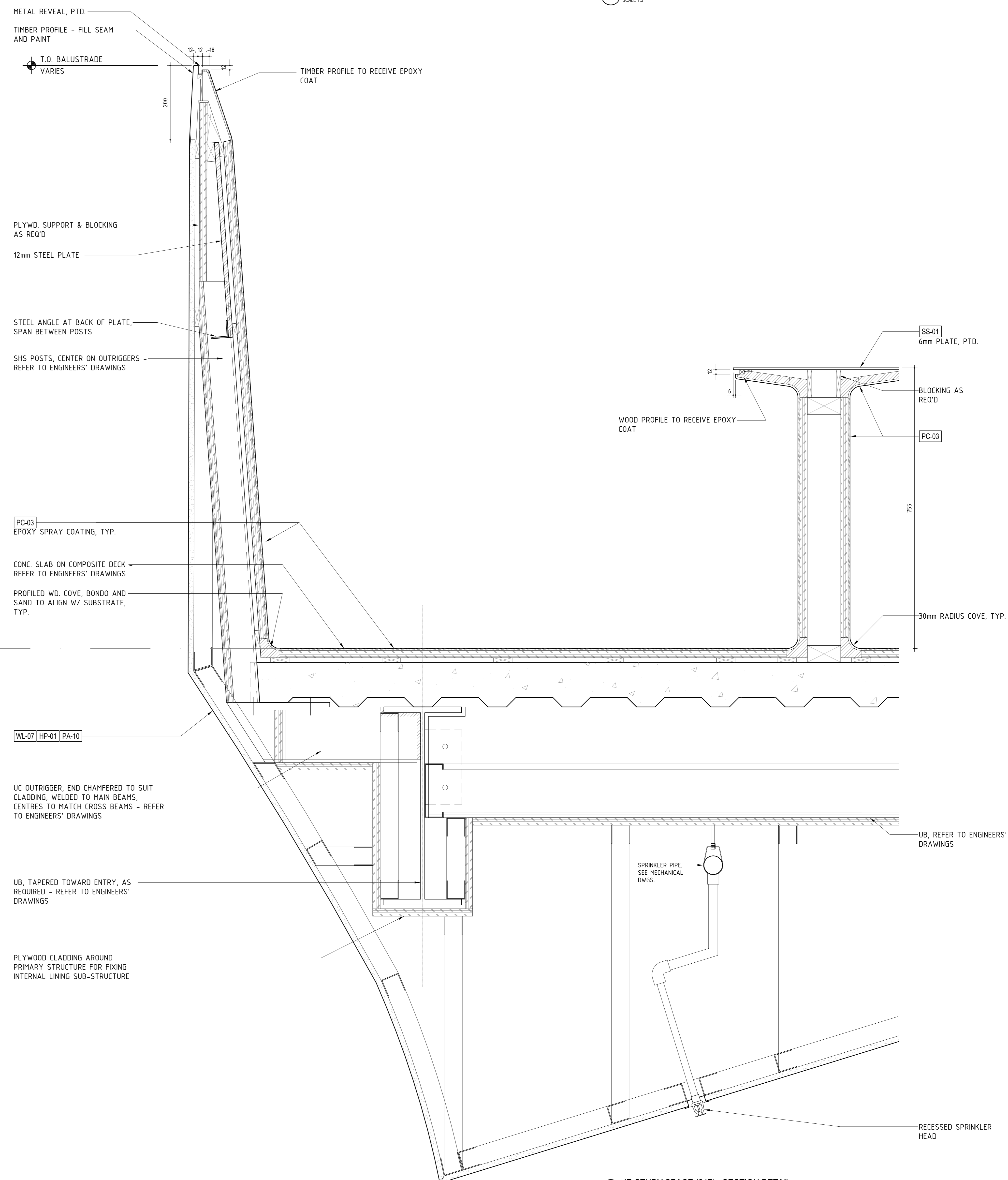
01 JR STUDY SPACE (247) - SECTION DETAIL SCALE 1:5
